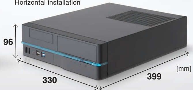
Horizontal installation
